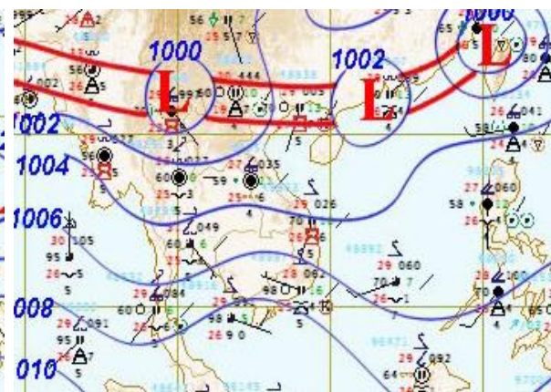
Figure 2: Weather map for 12 nd August 2016
