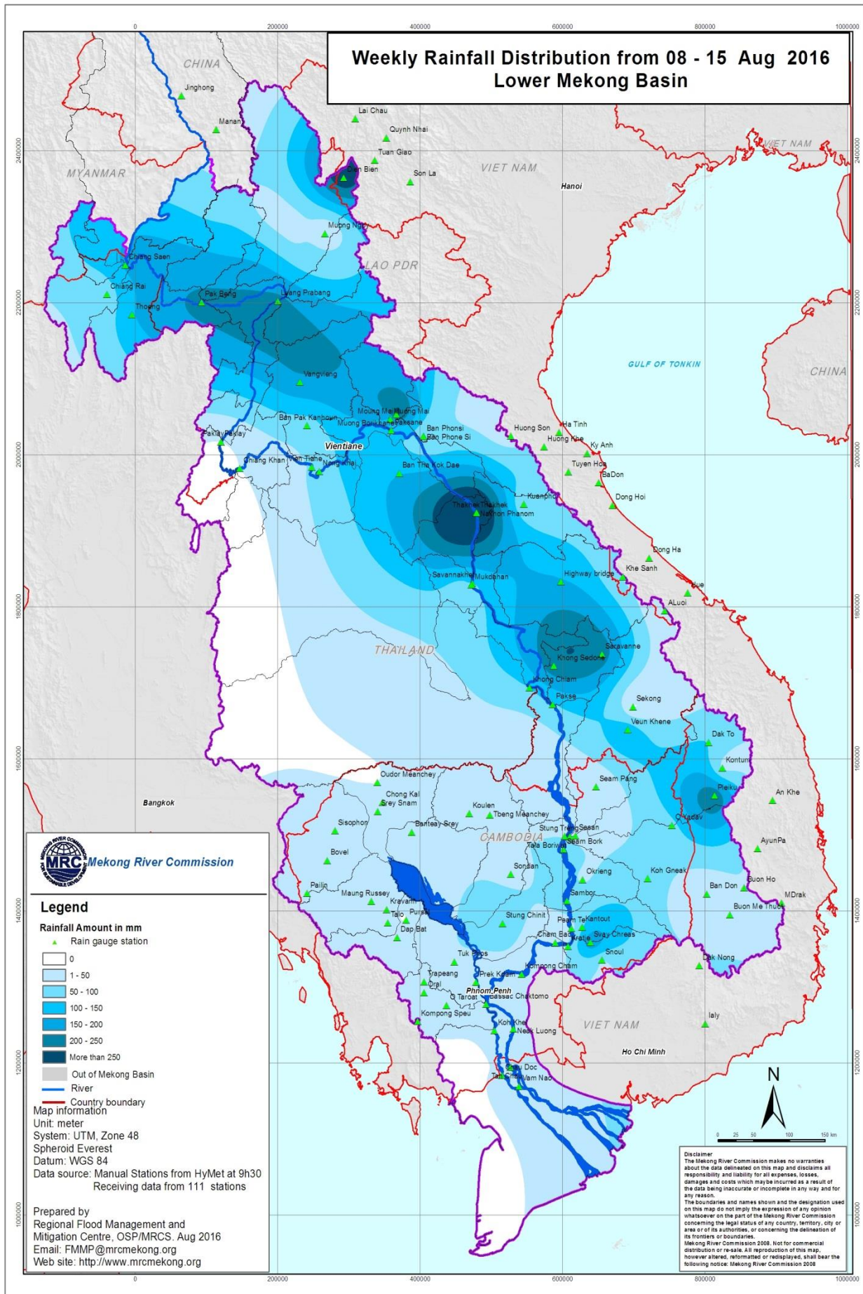
Figure 3: Weekly Rainfall Distribution over the LMB from 08 th – 15 th Aug, 2016
